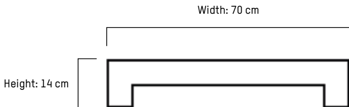
Excrement hole-slatted floor for sows in cross-section
